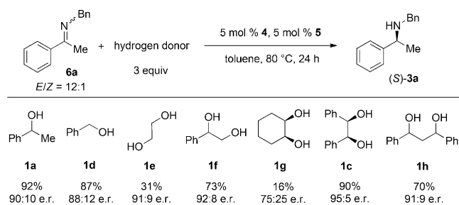
Scheme 2. Screening of hydrogen donors for ATH. The reactions were carried out under an N 2 atmosphere. The yield of (S)-3a was determined by GC using an internal standard. The e.r. value was determined by HPLC. See the Supporting Information for details.
