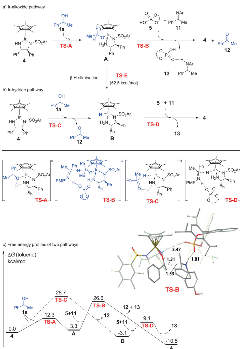
Figure 1. Free-energy profiles for the hydride transfer. TS = transition state.
